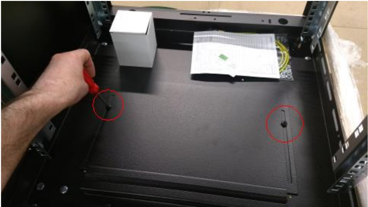
Picture showing bottom of rack and sliding access panel for cabling and services. Loosen the two screws to adjust panel gap required.
